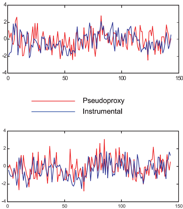
Figure 1. Sample ‘Pseudoproxy’ series for two gridpoint locations (top) 37.5N, 22.5E and (bottom) 12.5N, 32.5W from experiment 18A (Table 1) along with the associated actual instrumental annual-mean temperature series.
