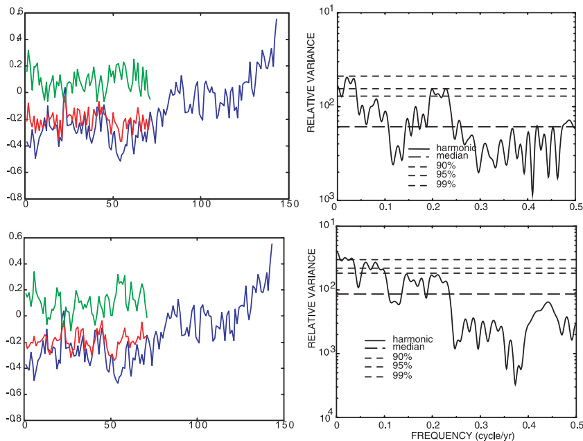
Figure 2. Global mean surface temperature reconstruction (red) along with actual infilled data (blue) for experiments 18A and 19A. Residuals are shown (green) along with the corresponding spectrum of residuals (right) based on multiple-taper procedure described by Mann and Lees [1996].
