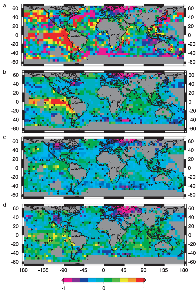
Figure 3. Actual (a) and Reconstructed Surface Temperature Anomaly Pattern (relative to 1961–1990 mean) for the year 1877 From Experiments 10B (b), 18A (c) and 18B (d), illustrating the influence of both SNR and the specific locations of pseudoproxies on the fidelity of the reconstructed pattern.
